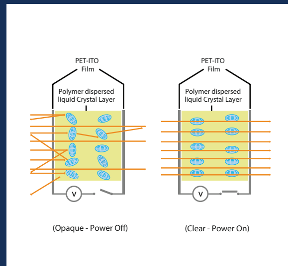
OPERATION PRINCIPLE
