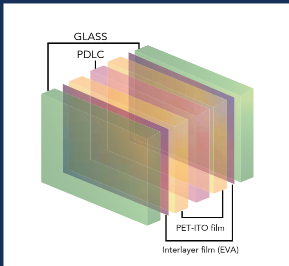
STRUCTURE
