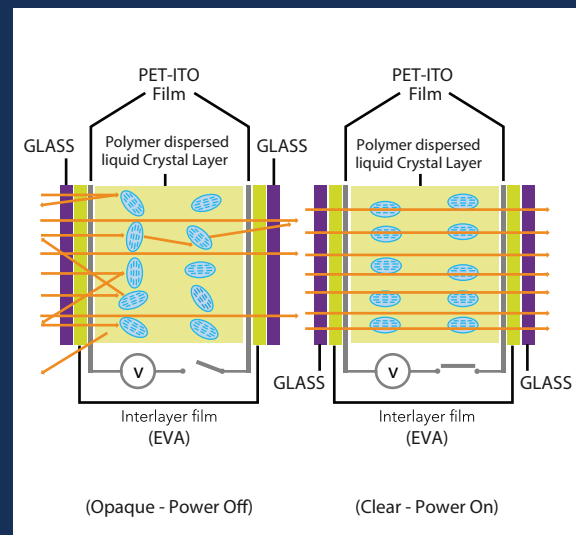
OPERATION PRINCIPLE
